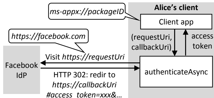
Figure 3.10: The data flow of authenticateAsync function in Modern app SDK
